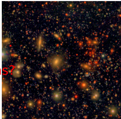
HSC image (COSMOS)
