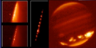
Shoemaker-Levy 9 (1994)
